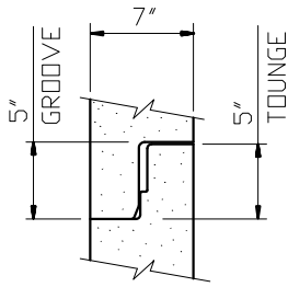
72" JOINT DETAIL
