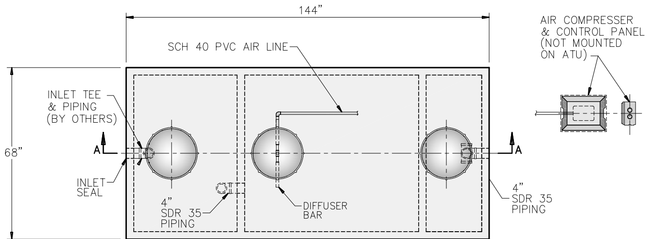
AEROBIC (1000 GPD) PLAN VIEW
