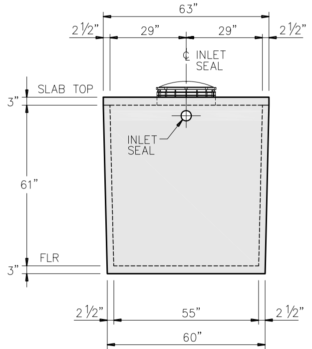
LEFT ELEVATION
