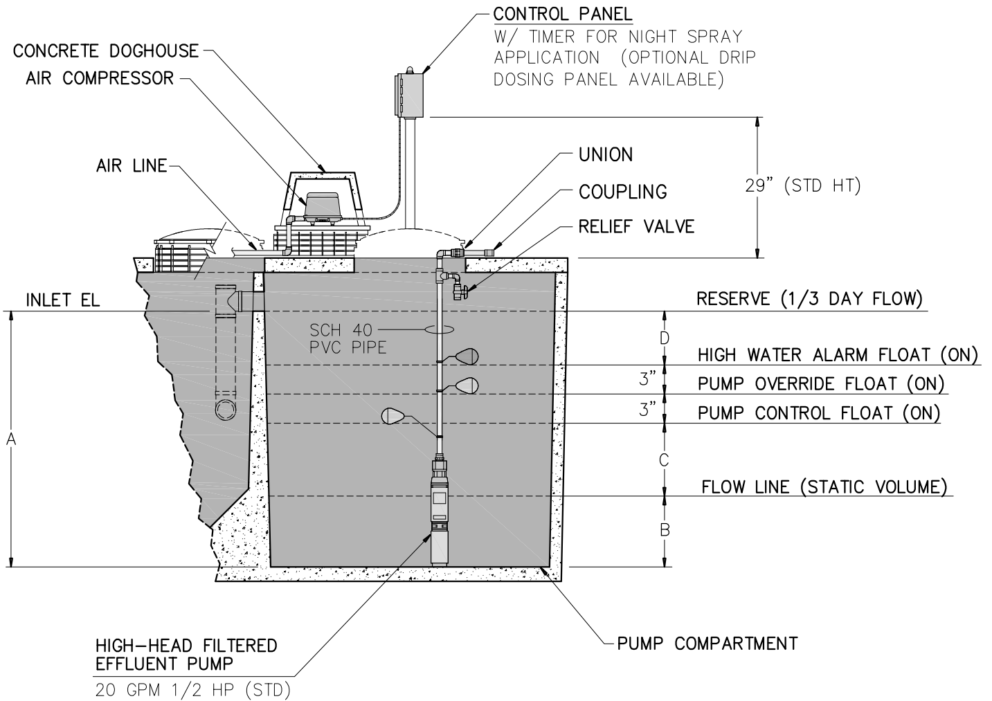
CUTAWAY SECTION (TO BE USED WITH ATU MODEL B-550 & B-800)
