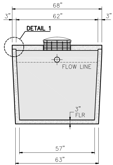
SECTION B-B
