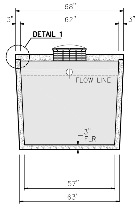
SECTION B-B
